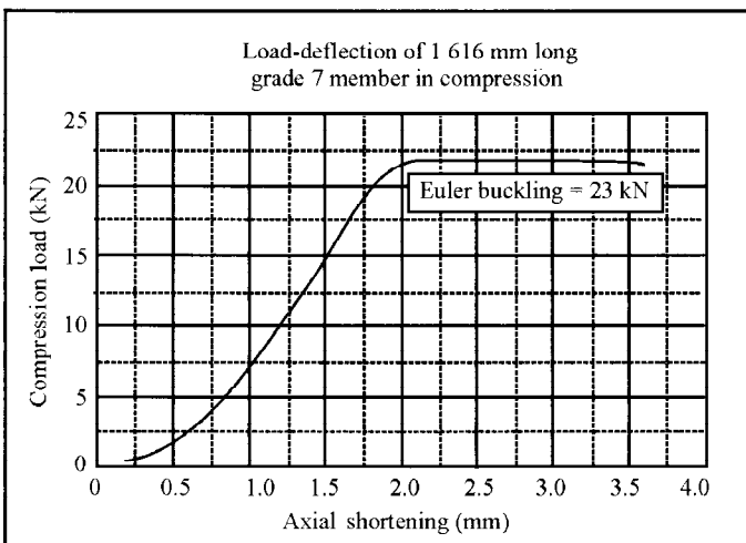
Figure 5 Compression strength of straight member or member with very little pre-curvature
