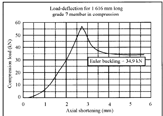
Figure 6 Compression strength of a straight member or member that has a bias to double curvature
