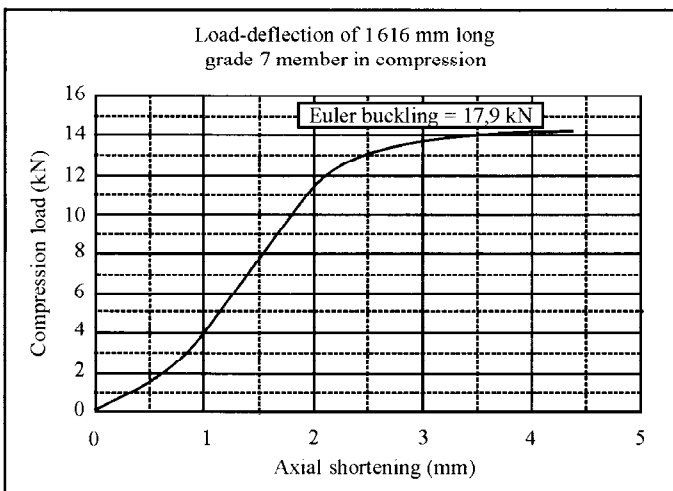
Figure 4 Compression strength of member with pre-curvature
