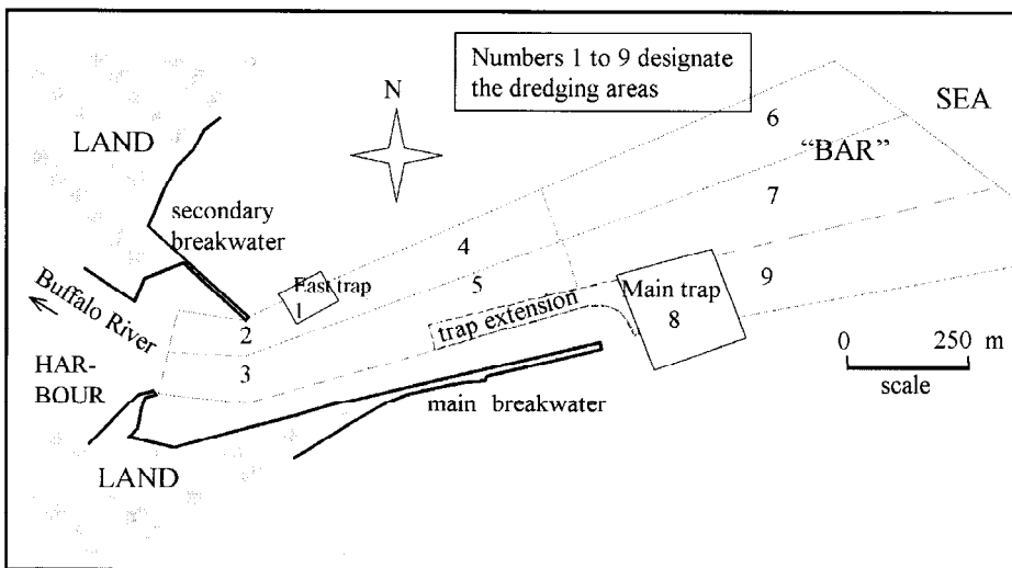
Figure 2 East London sand traps, breakwaters and dredging areas
